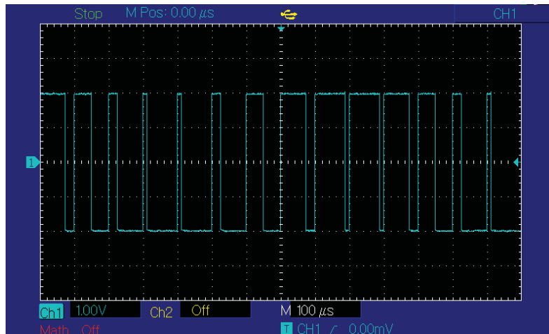
Figure 4- 30 Observe PWM waveform with oscilloscope
