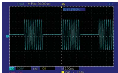
Figure 4- 3 Use channel output
