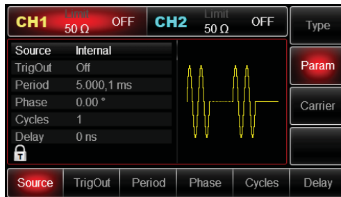
Figure 4- 56 Set period of pulse train
