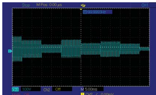
Figure 4-19 Observe QAM waveform with oscilloscope
