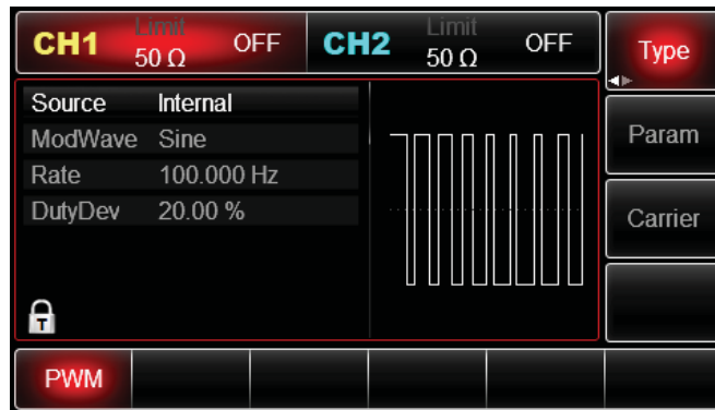
Figure 4- 20 Select PWM function
