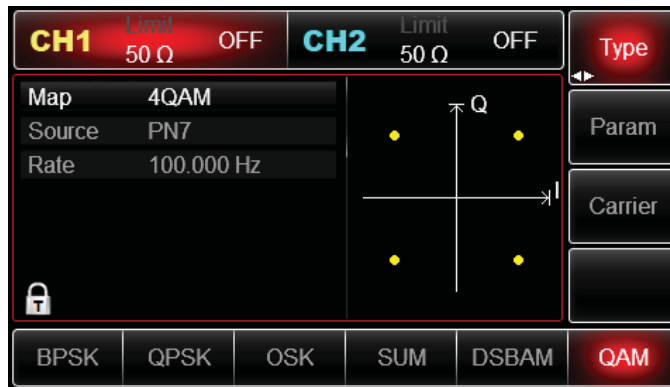
Figure 4-14 Select QAM function
