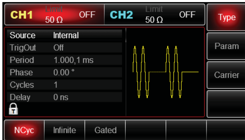
Figure 4- 52 Set N cycle function
