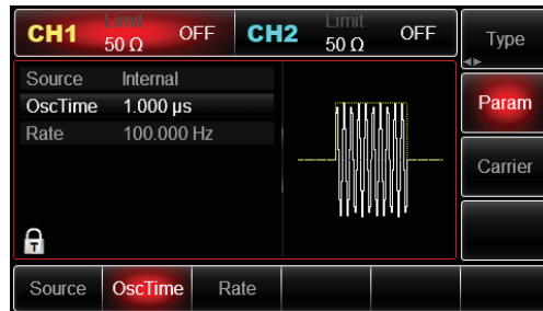
Figure 4- 2 Set modulation rate
