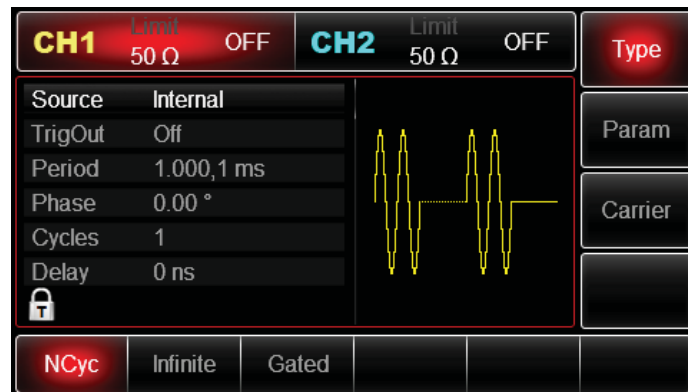
Figure 4-46 Select BURST function
