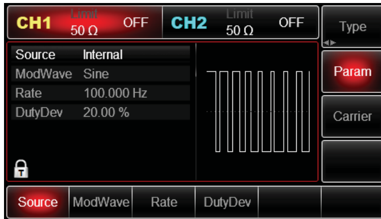
Figure 4-24 Set modulation parameters
