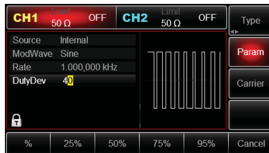
Figure 4-28 Set duty ratio deviation
