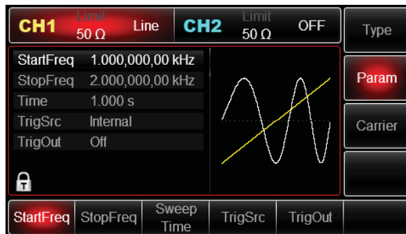
Figure 4- 33 Set frequency sweep parameters
