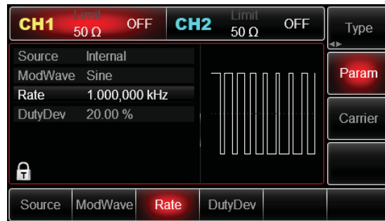
Figure 4- 27 Set modulation parameters
