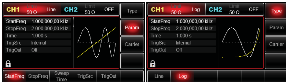
Figure 4- 35 Select logarithmic frequency sweep
