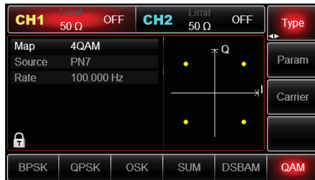
Figure 4- 12 Select QAM function
