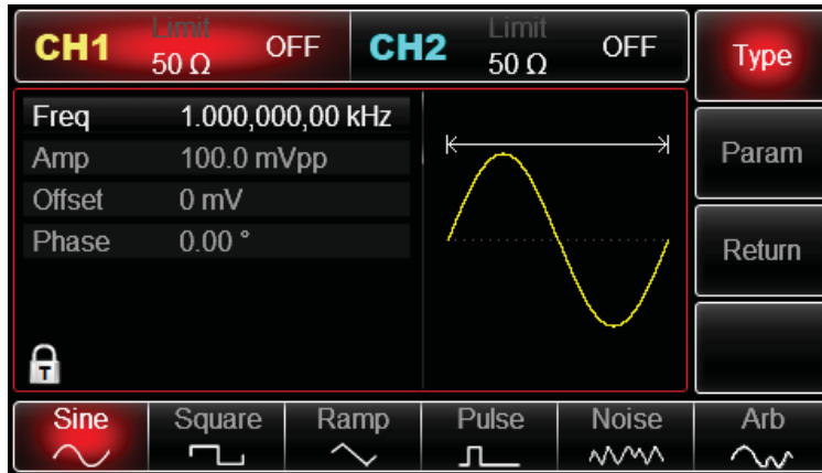
Figure 4-53 Select waveform of pulse train
