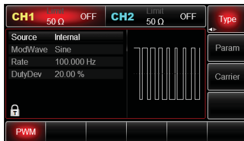
Figure 4-23 Select PWM function
