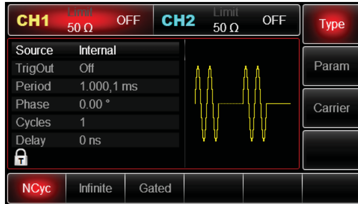
Figure 4-48 Select N cycle mode
