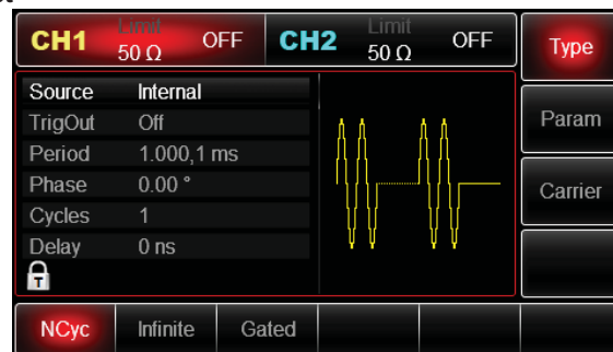
Figure 4-51 Set period of pulse train
