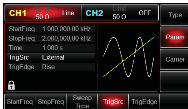
Figure 4- 38 Select external trigger source
