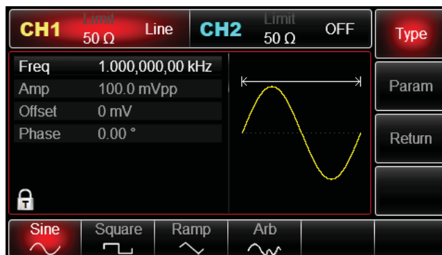
Figure 4- 32 Select frequency sweep waveform
