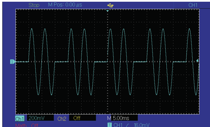
Figure 4-58 Observe BURST waveform with oscilloscope
