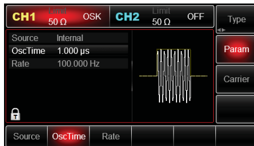
Figure 4- 3 Use channel output
