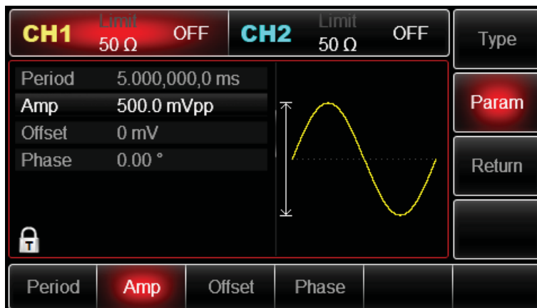
Figure 4-54 Set waveform amplitude
