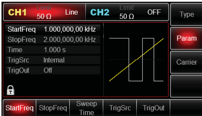
Figure 4-43 Set trigger frequency
