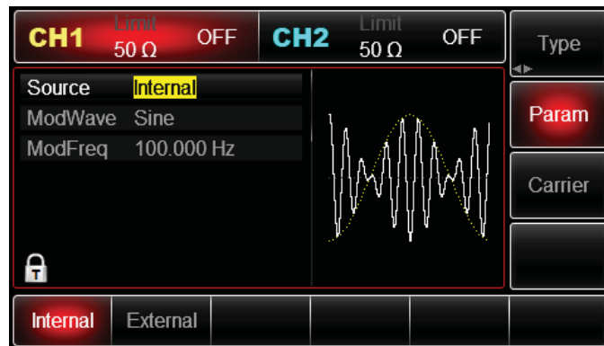
Figure 4- 10 Select modulation source
