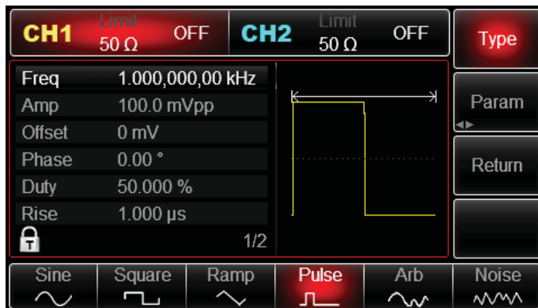
Figure 4-25 Set carrier parameters
