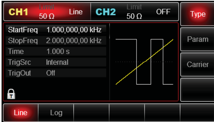
Figure 4-42 Set frequency sweep parameters
