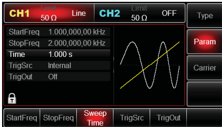
Figure 4- 36 Set frequency sweep time
