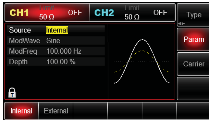
Figure 4- 6 Select modulation source
