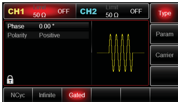
Figure 4-49 Select gating mode
